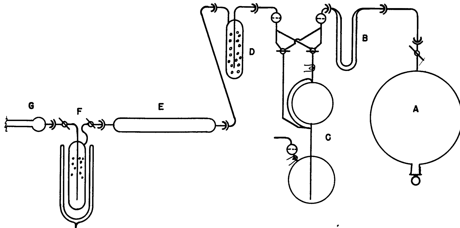
Fig. 8. Apparatus for purifying and isolating ethylene-d 4 .
